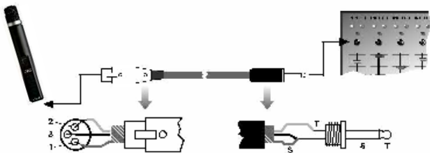
Figure 4: Connecting via an unbalanced cable
