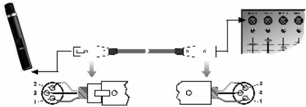
Figure 5: Connecting via a balanced XLR cable
