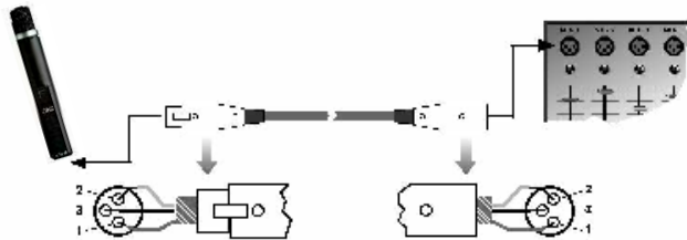
Figure 3: Connecting via a balanced XLR cable
