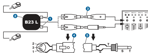
Figure 3: Using the B23 L to power the microphone
