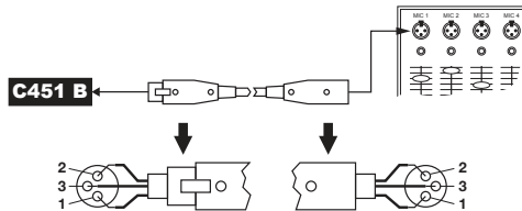
Figure 1: Connecting to a balanced input
