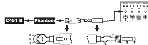
Figure 2: Connecting to an unbalanced input
