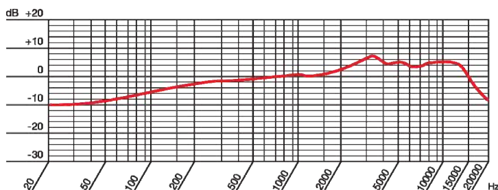
Frequency response trace:
