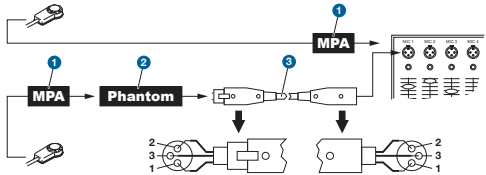
Figure 1: Connecting to balanced inputs
